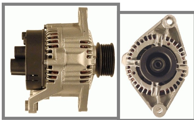
ALTERNATOR 12V,65A
