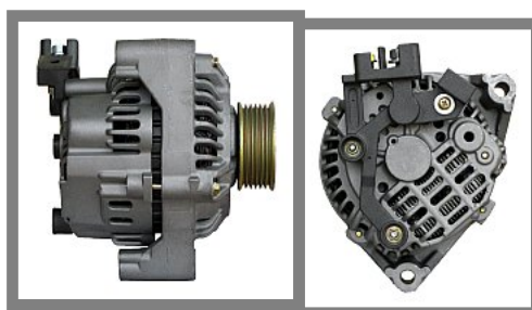
ALTERNATOR 12V,80A
